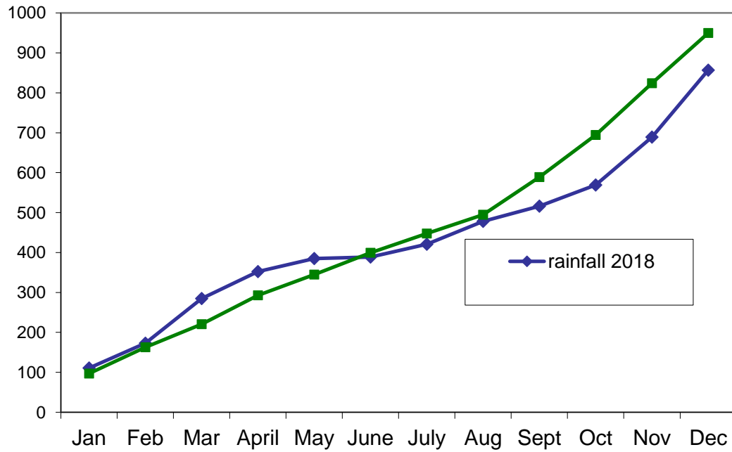
Cumulative Monthly Rainfall 2018 cf 10 year mean
